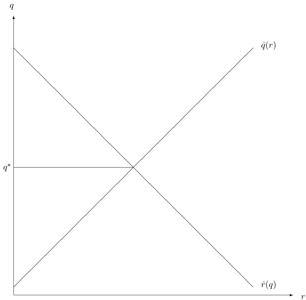
Figure 1: Best response diagram
