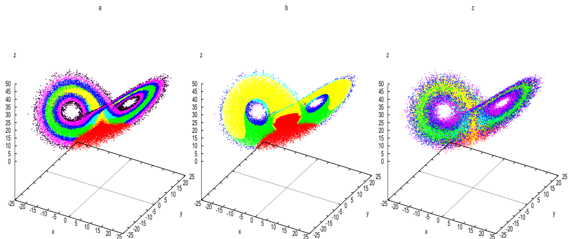
Figure 4. Views of the Lorenz attractor showing the doubling times for 2^{16} initial conditions for the Lyapunov direction (a), the maximum singular vector optimized for the doubling time obtained in the Lyapunov direction (b), and in random direction (c). Red indicates \tau_2 < 0.15 , yellow 0.15 \leq \tau_2 < 0.5 , green 0.5 \leq \tau_2 < 0.8 , turquoise 0.8 \leq \tau_2 < 1 , blue 1 \leq \tau_2 < 2 , magenta 2 \leq \tau_2 < 4 , and black for \tau_2 \geq 4 .
