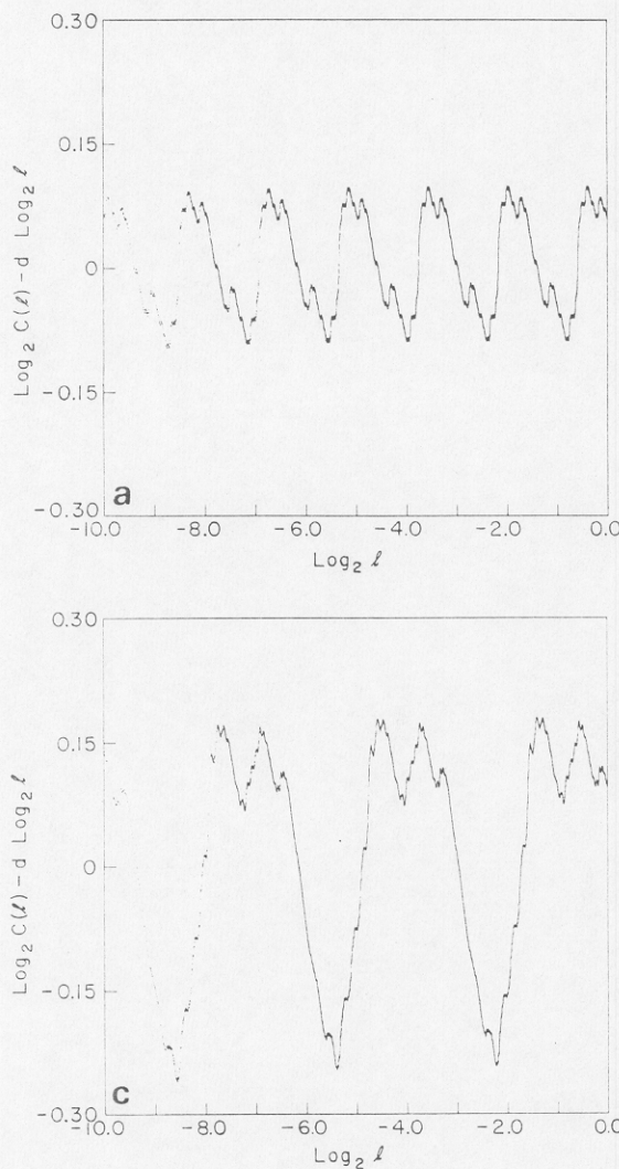
Fig. 2. Oscillatory residuals \psi for the sets (a) 101, (b) 101010001 and (c) 101001001.
