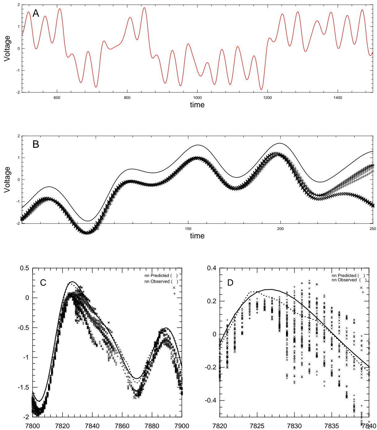
Figure 1: Four voltage series with related forecasts, for details see the text. A) A sample of the observations. B) Iterated ensemble forecasts using two different models. C) 15 step ahead forecasts of near recurrences. D) Zoom of C showing state-dependent systematic model error.
