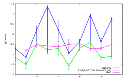
Figure 4: Ignorance as a function of lead time for the HadGEM2 and RAP models. The uncertainty bars are the 70th percentile from re-sampling from the forecast set. Lower values indicate better skill.
