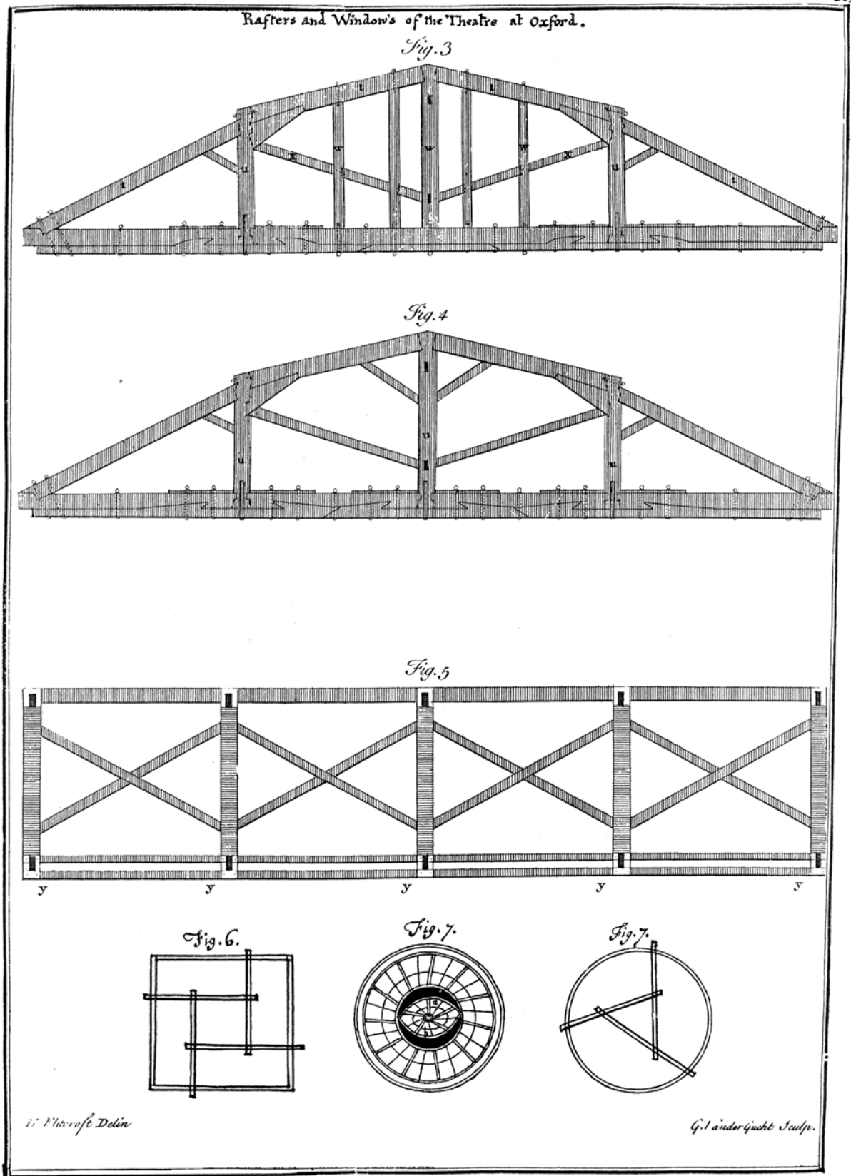
Fig. 8: The roof of the Sheldonian Theatre, Oxford as designed by Wren (Wren 1750, sect. XII, between p. 336 and p. 337).
