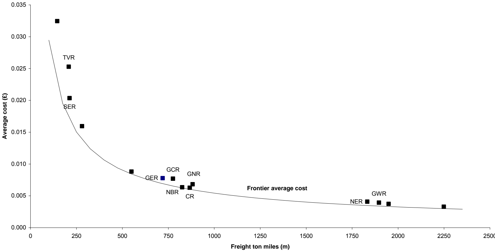
Freight ton miles - cost relationship, Britain's railways (1900)
